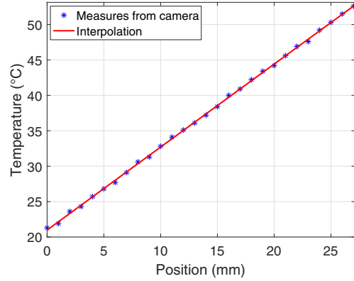
Fig. 5. Temperature measurements obtained from the thermographic camera on the aluminum bar during a test and respective linear interpolation.
