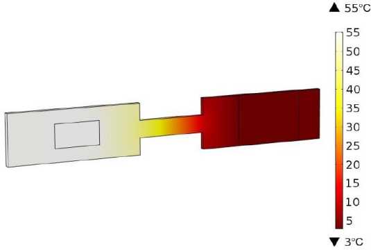
Fig. 2. FEM simulation of the temperature gradient on an aluminum bar with reduced-width in correspondence of the grating position.
