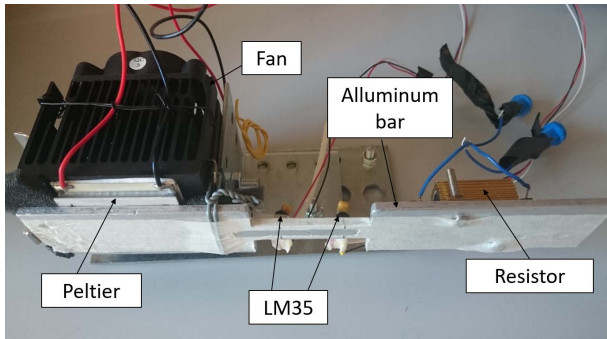
Fig. 3. The experimental setup. The picture also shows the position of the reference temperature sensors.
