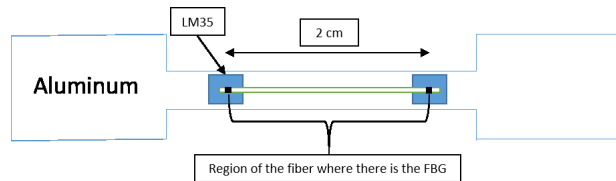
Fig. 6. Measurement set up for the single FBG.
