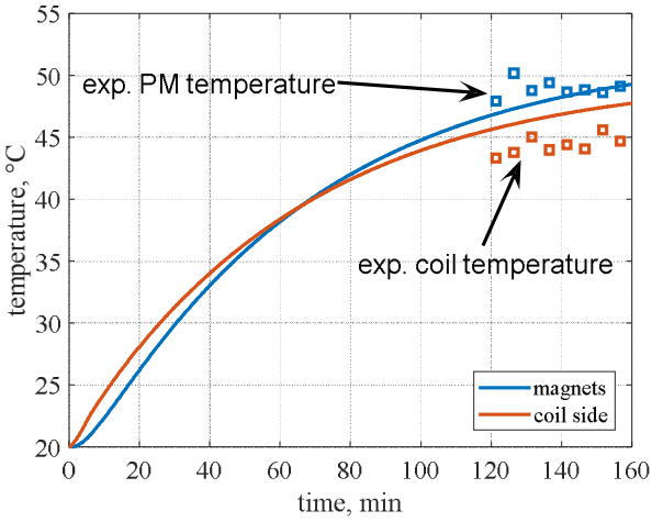
Fig. 5. Experimental validation of the thermal model: motor driven at 1500 rev/min at rated current.
