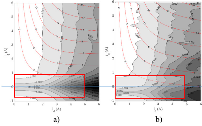
Fig. 11 k'_\epsilon contours: a) SyR; b) NdFeB-assisted SyR.
