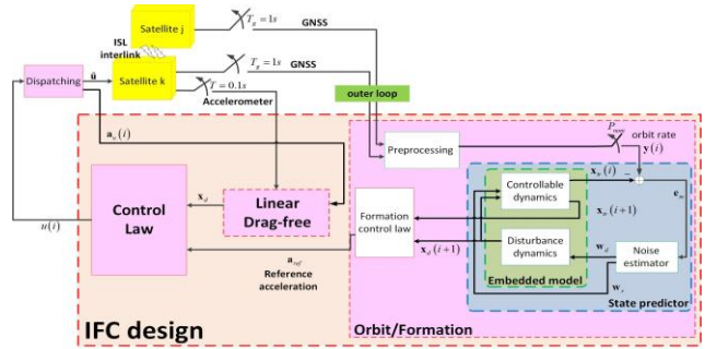
Fig. 3. Overall scheme of the IFC control unit.
