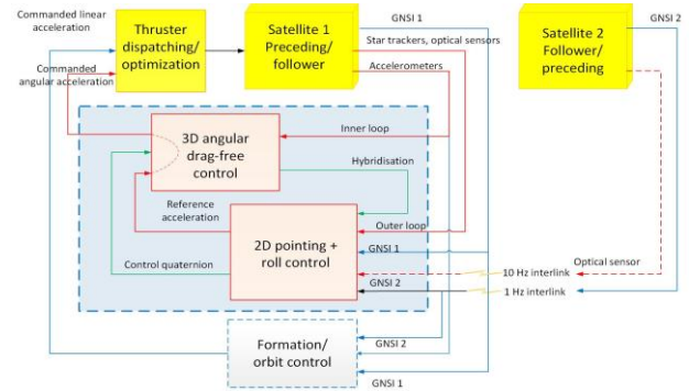
Fig. 4. Overall scheme of the attitude control unit.
