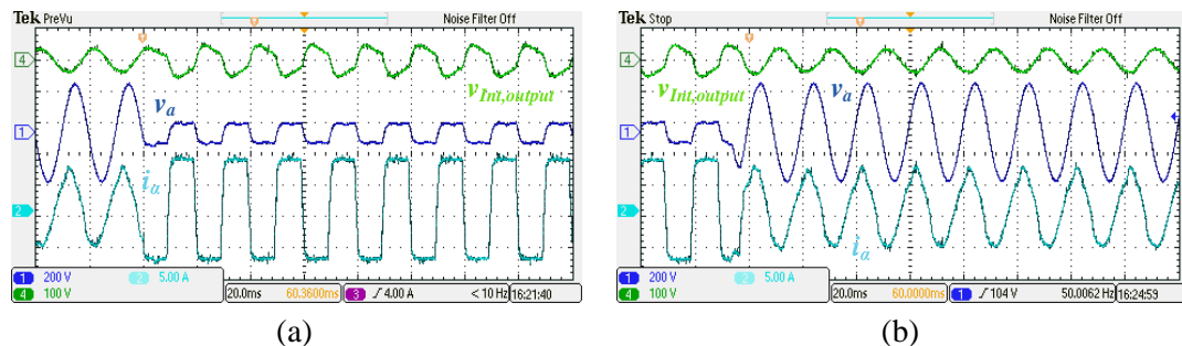
Fig. 4.37. Linear step load changing (100% - 95% and viceversa) - integral output (100 V/div), real capacitor voltage (200 V/div) and real inductor current (5 A/div) ( \alpha -axis), time scale (20 ms/div): (a) from rated load (68 \Omega ) to overload conditions (7.2 \Omega ); (b) from overload conditions (7.2 \Omega ) to rated load (68 \Omega )
