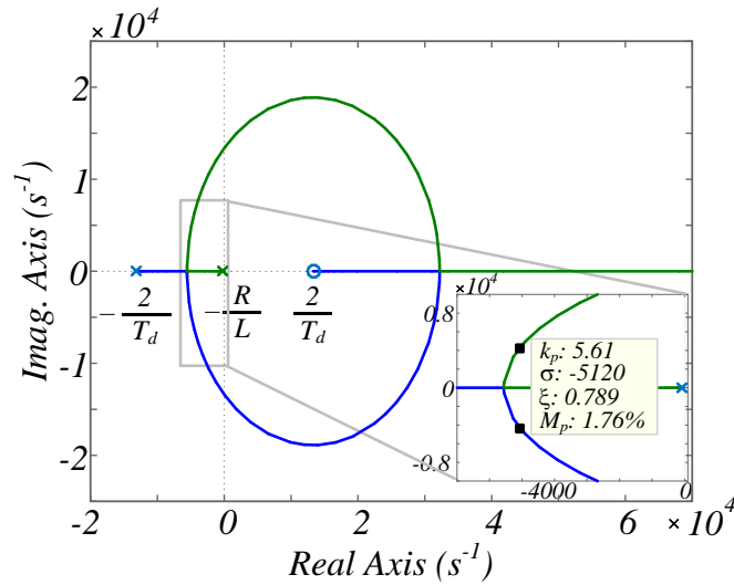
Fig. 3.15 Root locus for the inner current loop with P regulator and with ideal voltage decoupling : x – open loop poles; ■ closed-loop poles for k_{pI} = 5.61 ; o – zeros; G_{PWM}(s) = (1 - T_d s/2)/(1 + T_d s/2)
