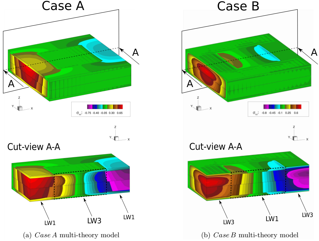
Figure 4: Composite four-layered plate. Transverse shear stress \sigma_{xz} . Multi-model theories.
