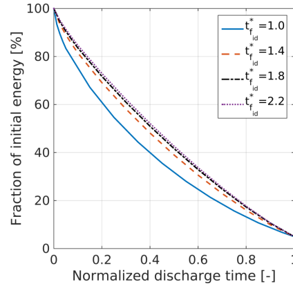
Figure 16. Normalized energy history during the discharge for the 4 optimized designs
