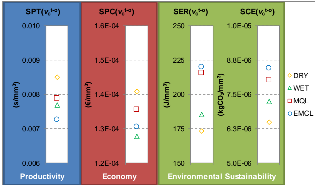
Figure 45. Influence of lubricating/cooling condition on productivity, economy, and environmental sustainability when turning Ti-6Al-4V at the cutting speed for trade-off criterion.
