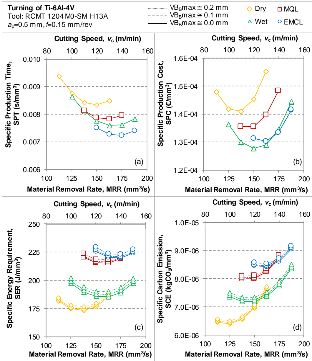
Figure 42. Specific production indicators (SPT (a), SPC (b), SER (c), and SCE (d)) when turning of Ti-6Al-4V under various lubrication/cooling condition. Note: the curves for SPC at different VB_B \text{max} are basically overlapped.
