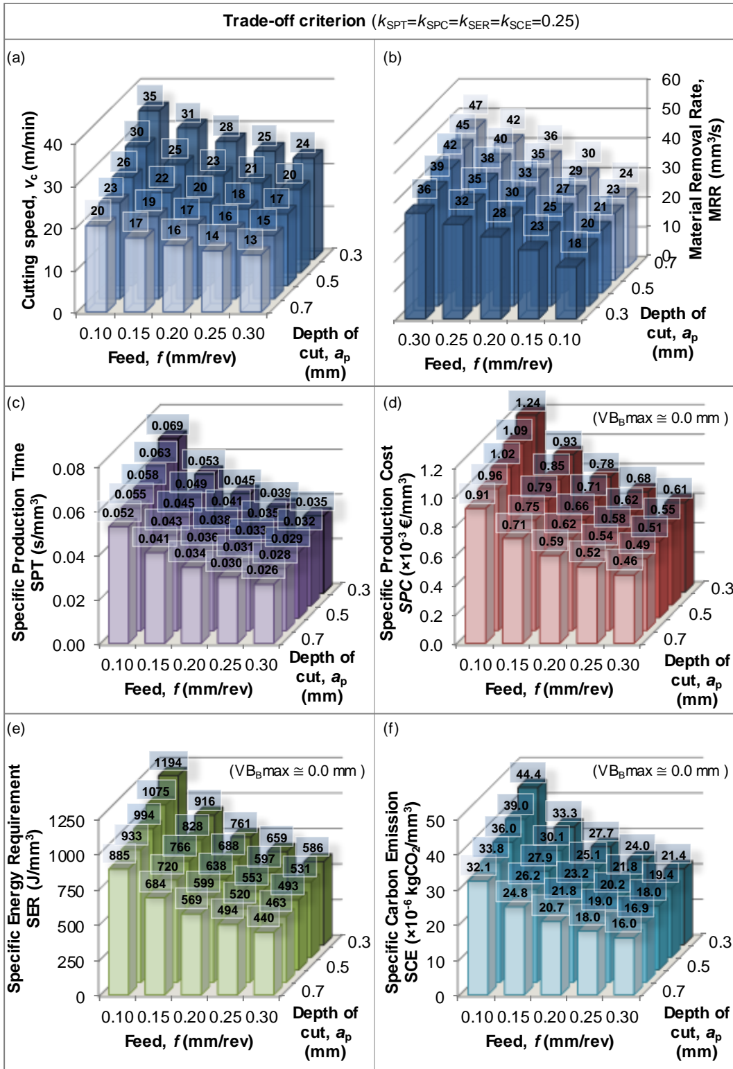
Figure 18. Cutting speed (a), Material Removal Rate (b), SPT (c), SPC (d), SER (e), and SCE (f) for the trade-off criterion.
