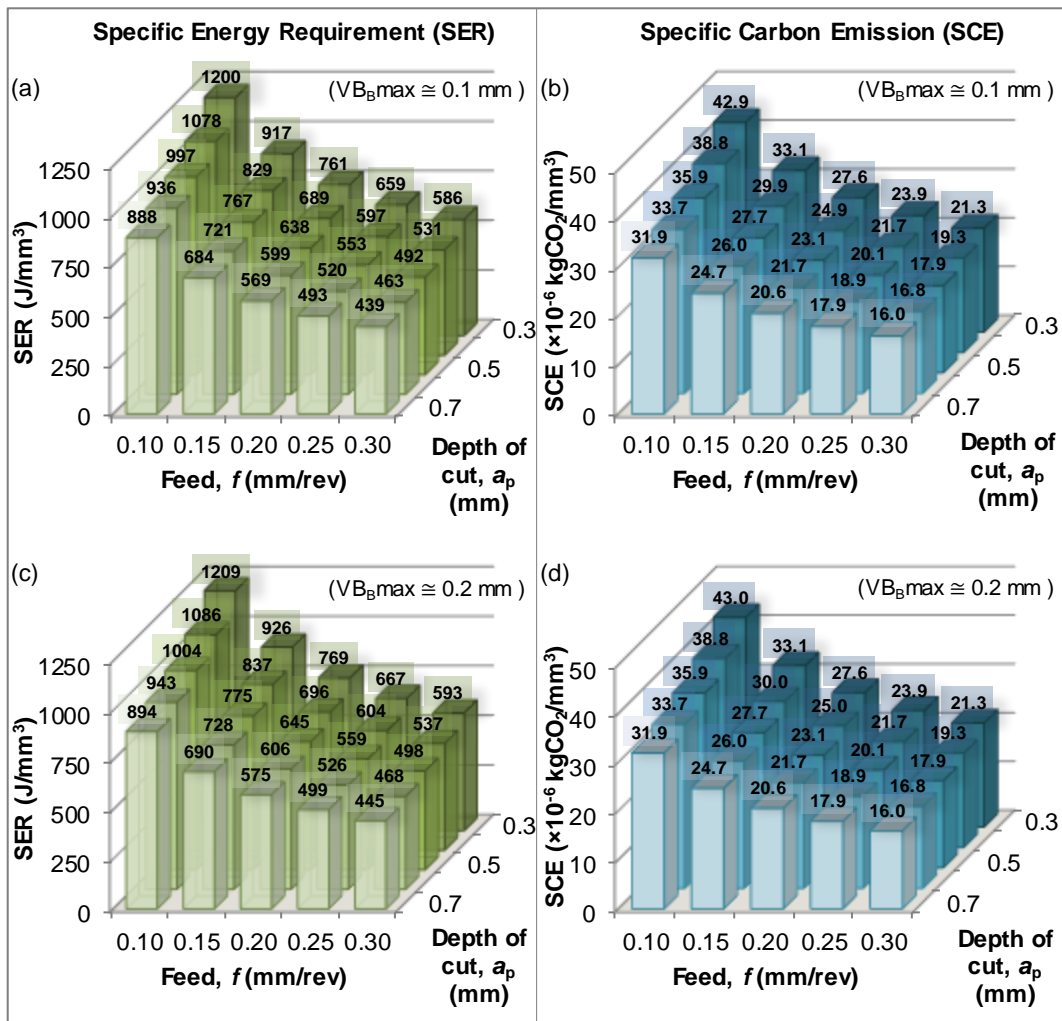
Figure 17. Specific production indicators SER and SCE for VB_{Bmax} \approx 0.1 \text{ mm} (a, b) and VB_{Bmax} \approx 0.2 \text{ mm} (c, d).
