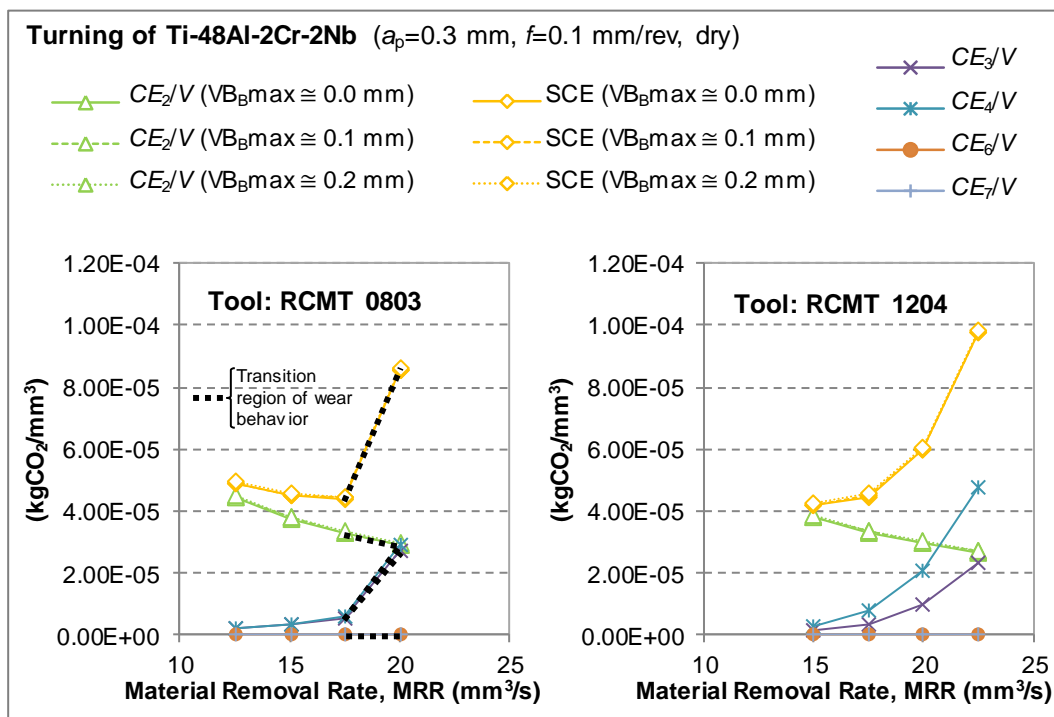
Figure 24. Specific Carbon Emission and its contributions as a function of cutting tool.
