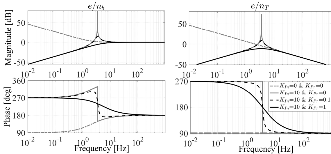
Fig. 13. Bode plots for transfer functions \frac{e(s)}{n_b(s)} (left) and \frac{e(s)}{n_T(s)} (right)
