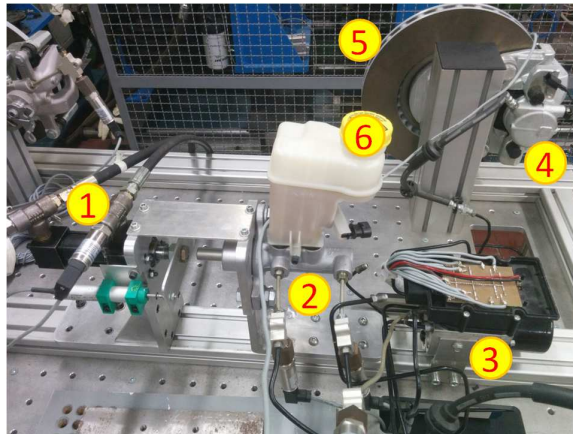
Fig. 2. HIL Test Rig 1-Hydraulic cylinder 2-TMC 3-customized ESC 4-Brake caliper 5-Brake disk 6-oil tank
