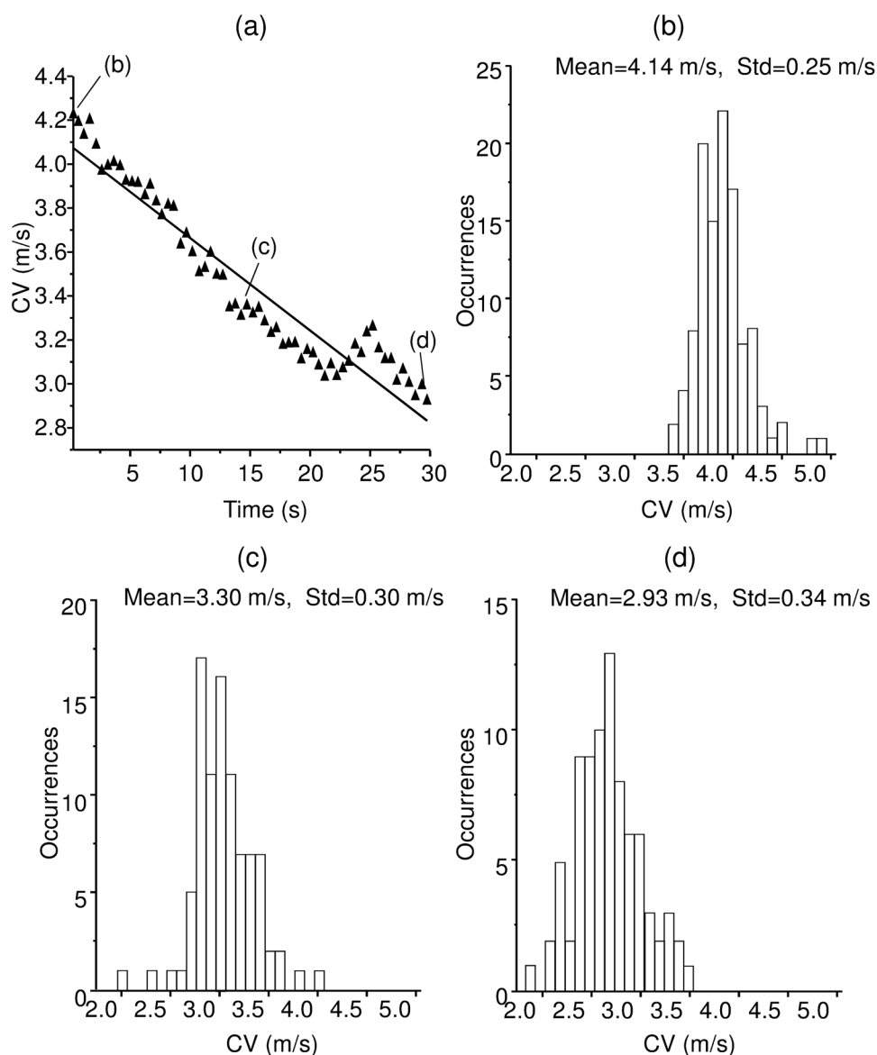
Figure 1. (a) Global CV estimates and (b)–(d) CV distributions obtained from EMGs detected during a 30s long constant force (60% MVC) isometric contraction of a healthy biceps-brachii. Global CV was estimated using the method described in McGill and Dorfman (1984) whereas CV distributions were calculated from 1s epochs using the method described in Farina et al (2000). It can be observed that global estimate and its changes are in agreement with those provided by the estimation of CV distribution. Adapted from Farina et al (2000) with permission.
