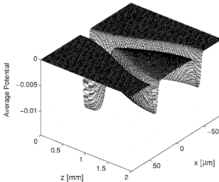
FIG. 4. Behavior of the cycled-averaged potential V_{av}(x, y, z) , taken at y=0^+ , along the adiabatic section of the optical waveguide.
