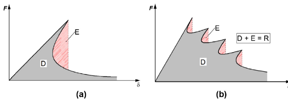
Figure 2. Load–displacement curves representing (a) a catastrophic failure (single snap-back) and (b) a global softening behavior perturbed by multiple local instabilities (snap-backs). The grey areas identify the dissipated energy, D , whereas the red (dashed) ones represent the emitted energy, E . The total released energy, R , is the summation of the two previous areas: D + E = R . Reproduced with permission from [7], Elsevier, 2016.
