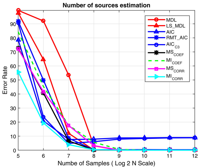
Fig. 6 Error rate for our proposed algorithm as well as algorithms presented in Table 1 versus number of samples at SNR = -5 dB
