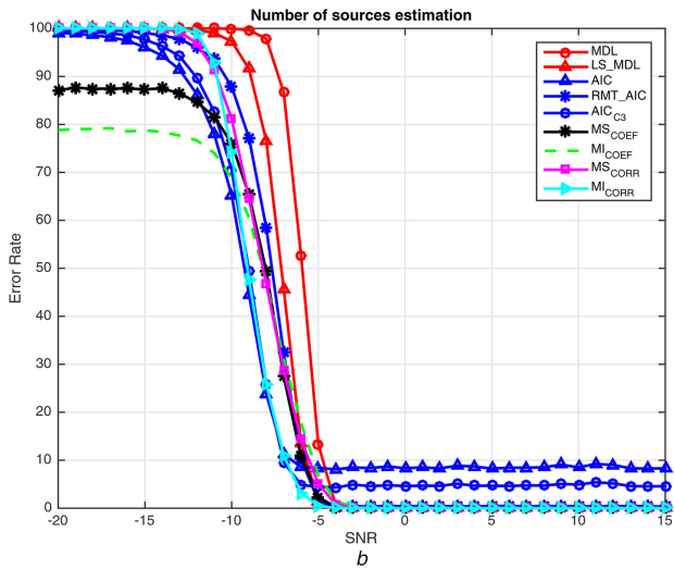
Fig. 5 Error rate for our proposed algorithm as well as algorithms presented in Table 1 versus SNR at (a) N = 1024 samples and (b) N = 100 samples
