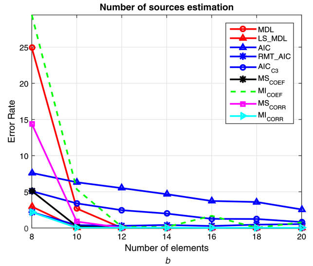
Fig. 7 Error rate for our proposed algorithm as well as algorithms presented in Table 1
