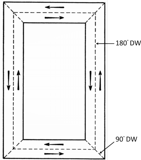
Fig. 2.5 A simple domain structure in a single crystal of Fe-Si (adapted from [36]). The rotation of magnetic field from one limb to another is controlled by four 90^\circ domain walls (dashed oblique segments) existing in each of the four corners of the crystal. The arrows indicate the direction of local polarization.
