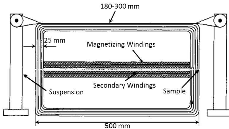
Fig. 3.12 Single Sheet Tester recommended by IEC 60404-3 adapted from [48]. The pole face is 25mm thick. The primary and secondary windings should be at least 440mm long. The primary winding can be a single layer, made of 1mm diameter wire with 400turns. The number of secondary windings is not fixed, and is suited to accurate signal acquisition.
