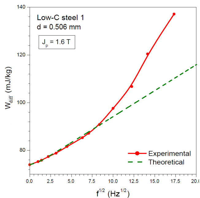
Fig. 6.15 The quantity W_{diff} = W_{tot} - W_{cl} vs. \sqrt{f} for a 0.506 mm thick LCS-1 at J_p=1.6 T (dots) along with the theoretical W_{diff} = W_{hyst} + W_{exc} (dashed line) where Eq. 6.21 is applied to compute the excess loss. Again, a deviation between the experimental and theoretical results is observed beyond 60 Hz due the appearance of skin effect.
