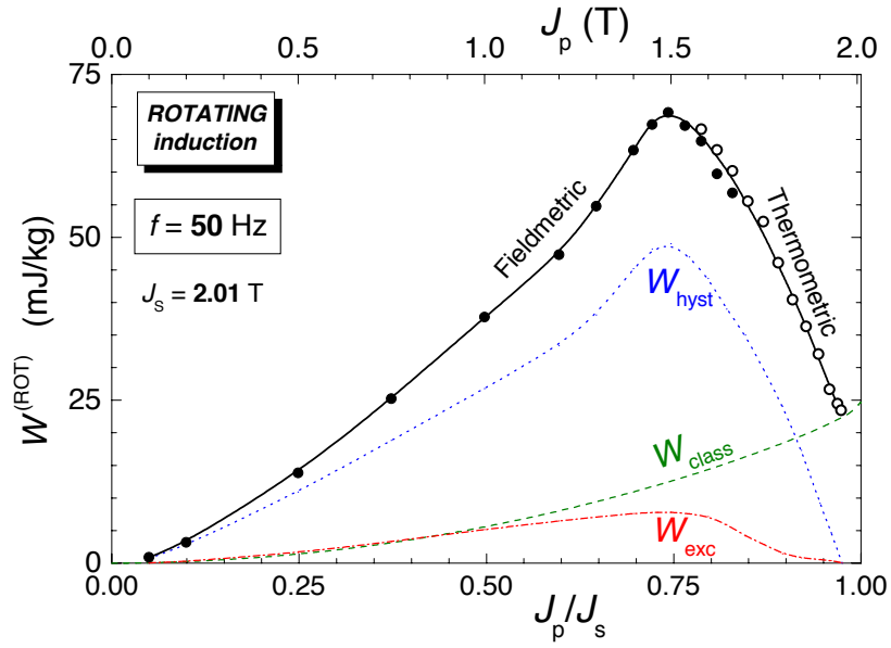
Fig. 5.5 Separation of loss obtained under rotating induction at 50Hz. The components W_{hyst} and W_{exc} vanishes at J_p/J_s \approx 0.98 as the total loss approaches to W_{class} .
