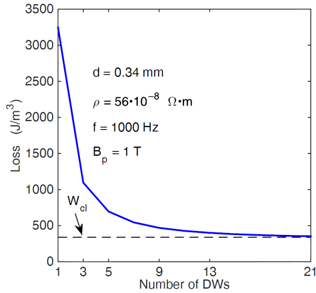
Fig. 2.8 Total loss vs. number of domain walls for a 0.34mm thick and 2mm long slab obtained by numerical simulation. It can be seen that the loss decreases with increase in the number of domain walls and ultimately becomes equal to the classical loss (Eq. 2.14).
