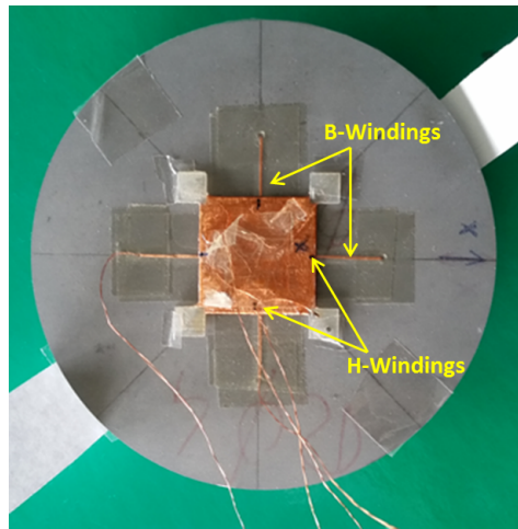
Fig. 3.17 B -Windings threaded through the sample through holes drilled in the sample. These windings are placed orthogonal to each other to measure the field in x and y directions. H -sensor is placed very close to the surface to measure H at its surface with double windings along x and y direction.
