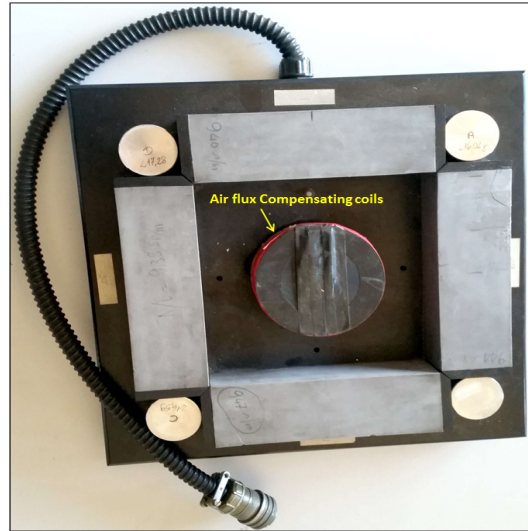
Fig. 3.9 A 700 turns compensated Epstein frame. The standard weights are placed at each corner. The samples cut along the transverse and rolling directions should be loaded into the opposite limbs.
