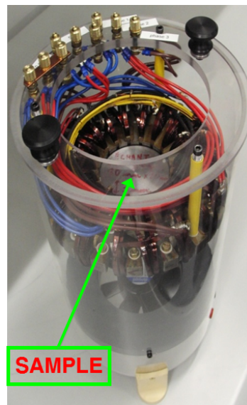
Fig. 3.18 The high frequency low induction magnetizer with sample placed in its center toroidal winding configuration as shown in Fig. 3.19. The core was assembled by using 0.35 mm thick non-oriented Fe-Si sheets.
