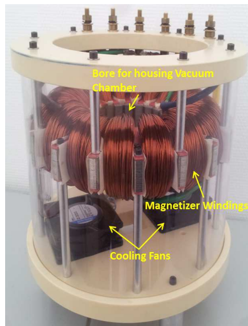
Fig. 3.20 High induction magnetizer designed to perform analysis at high inductions close to saturation conditions. The bore of the magnetizer can accommodate a cylindrical plexiglas vacuum chamber to achieve adiabatic conditions.
