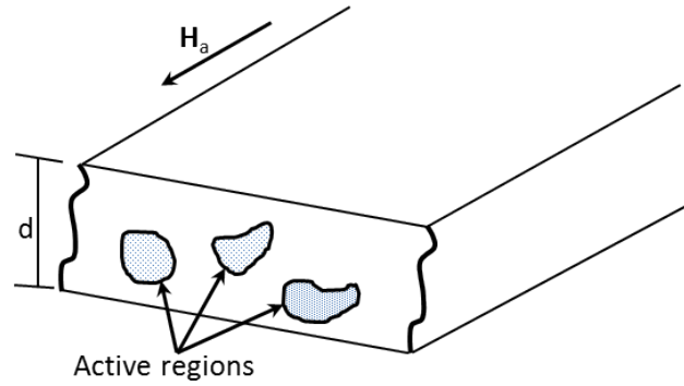
Fig. 2.10 Magnetic objects randomly distributed in a material that play the same role as active domain walls but with different eddy current damping effects due to different internal structures. MOs have different structural and dynamic properties in different materials.
