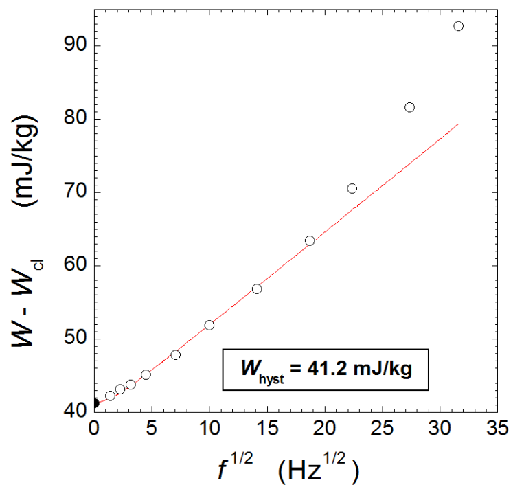
Fig. 2.2 The quantity W - W_{cl} at different frequencies obtained in a 0.35mm thick Fe-(3.2wt%)Si at B_p = 1.55 T under 1D flux. The measurements have been extrapolated up to f = 0 Hz to obtain W_{hyst} .
