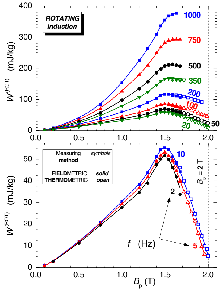
Fig. 5.3 Energy loss vs. peak induction in the frequency range (2 Hz- 1 kHz) under rotational flux. As in Fig. 5.2, measurements are carried out by applying both fieldmetric and thermometric methods and a region exists where the solid and the open symbols overlap.
