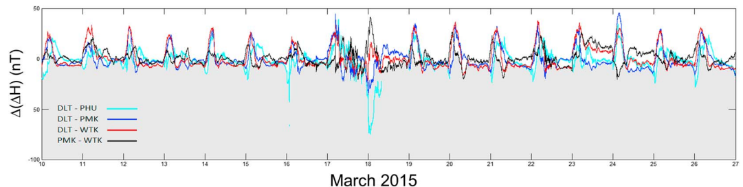
Figure 4. Differentiated \Delta H for the couples DLT-PHU (light blue line), DLT-PMK (blue line), DLT-WTK (red line), and PMK-WTK (black line).
