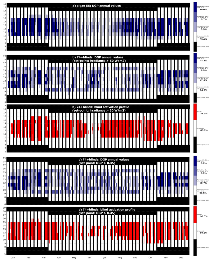
Fig. 6. Annual DGP values in the same room equipped with the algae-system and with a traditional venetian blind. Results for Turin.
