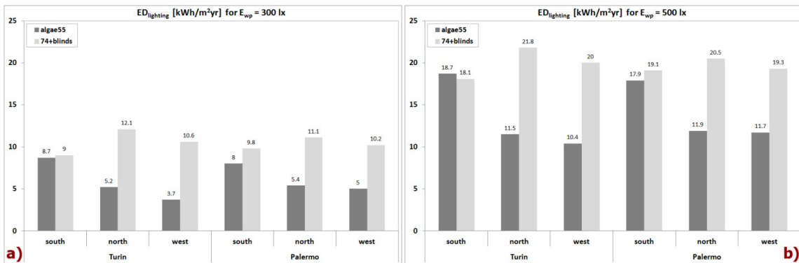
Fig. 7. Comparison of the daylight amount in the same room equipped with the algae-system and with a traditional venetian blind: results in terms of energy demand for lighting ED l for a work plane illuminance of 300 lx (a) and of 500 lx (b).
