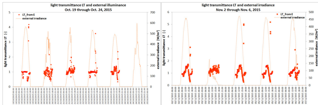
Fig. 4. Example of illuminance data recorded for two weeks and of the corresponding LT calculated. External irradiance are also plotted to allow sky conditions to be identified (clear vs. overcast).
