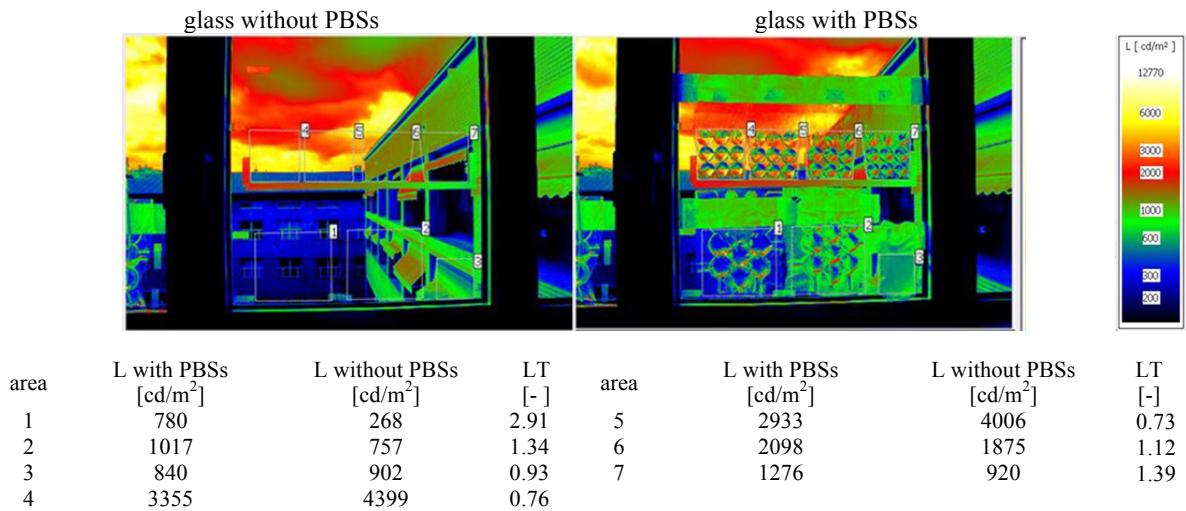
Fig. 3. Example of luminance maps recorded for one day and of the corresponding LT calculated.
