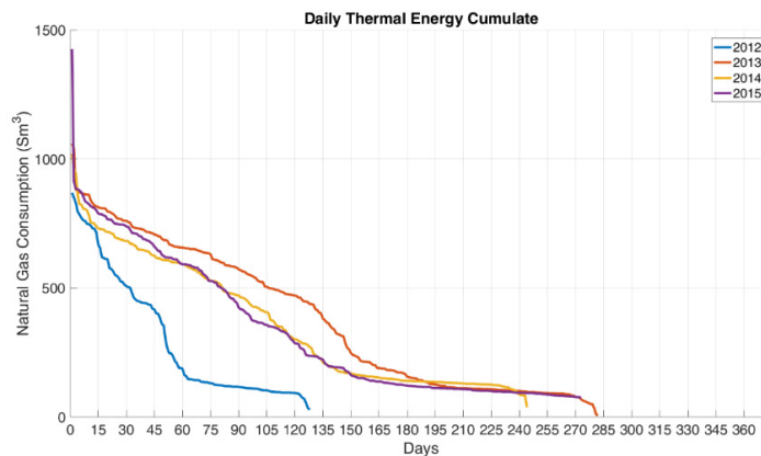
Figure 8. Office O2 - Daily natural gas consumption cumulate.
