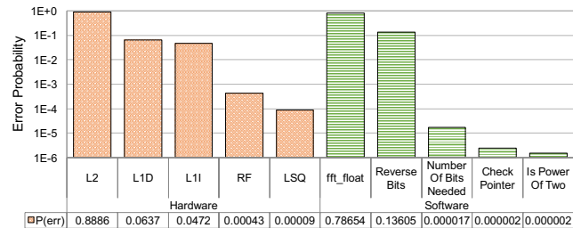
Figure 12: Example of diagnostic analysis for the x86 fft configuration.
