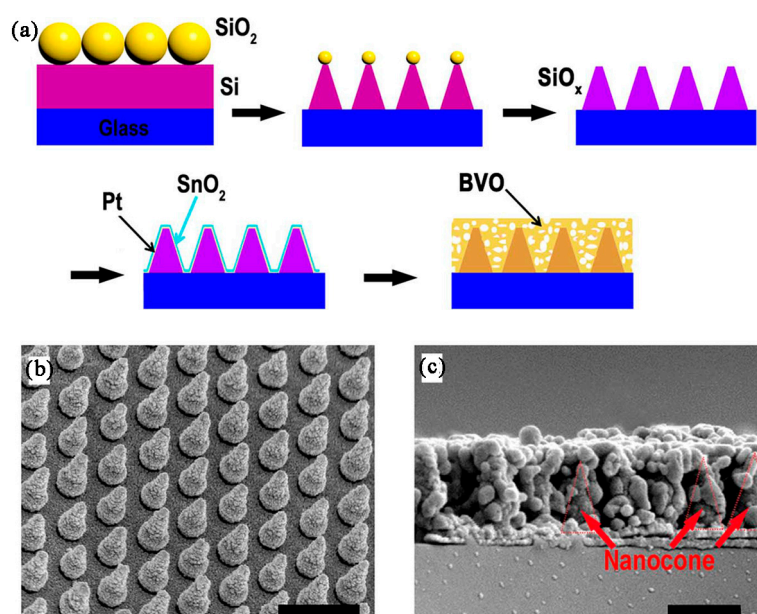
Figure 6. Pt/ \text{SnO}_2 / \text{Mo:BiVO}_4 on an engineered nanocone substrate. (a) Schematic illustration of the fabrication process of the conductive nanocone substrate; (b) scanning electron microscope (SEM) image ( 60^\circ tilting) of the final \text{SiO}_x /Pt/ \text{SnO}_2 nanocone arrays; (c) cross-sectional SEM images of \text{Mo:BiVO}_4 on the \text{SiO}_x /Pt/ \text{SnO}_2 nanocone substrate. Some exposed nanocones were also marked in the figure (c). Scale bars, 500 nm. Images adapted and used under Creative Commons CC-BY-NC license, attributed to [90]. Reprinted with permission of from [90]. Copyright American Association for the Advancement of Science, 2016.
