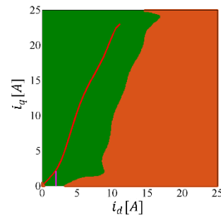
Fig. 15. Stable (green) and unstable (brown) regions at zero and low speed. Red: MTPA. Magenta: minimum flux limit.
