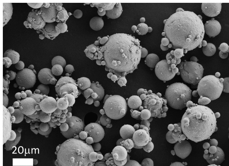
Figure 2. Field Emission Scanning Electron Microscopy (FESEM) image of gas atomized aluminum powders: the particles are spherical and their size varies between 1 and 30 µm.
