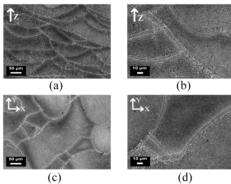
Figure 9. Optical micrographs of AlSi10Mg samples obtained by means of DMLS, built using a rotated scanning strategy ( 67^\circ of rotation between subsequent layers), at different magnifications: (a,b) describe a vertical section of the part along the building direction ( z axis); while (c,d) show the section parallel to the building plane ( xy -plane).
