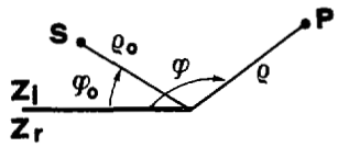
Fig. 1 . Geometry of the problem and transmission line representation.
