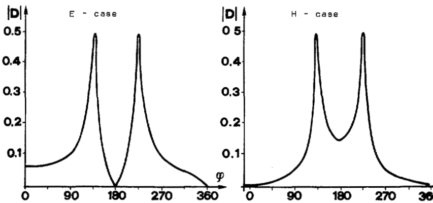
Fig.2 . Diffraction coefficients for \varphi_0=45^\circ , Z_1=0 and K_0 \rho_0=50
