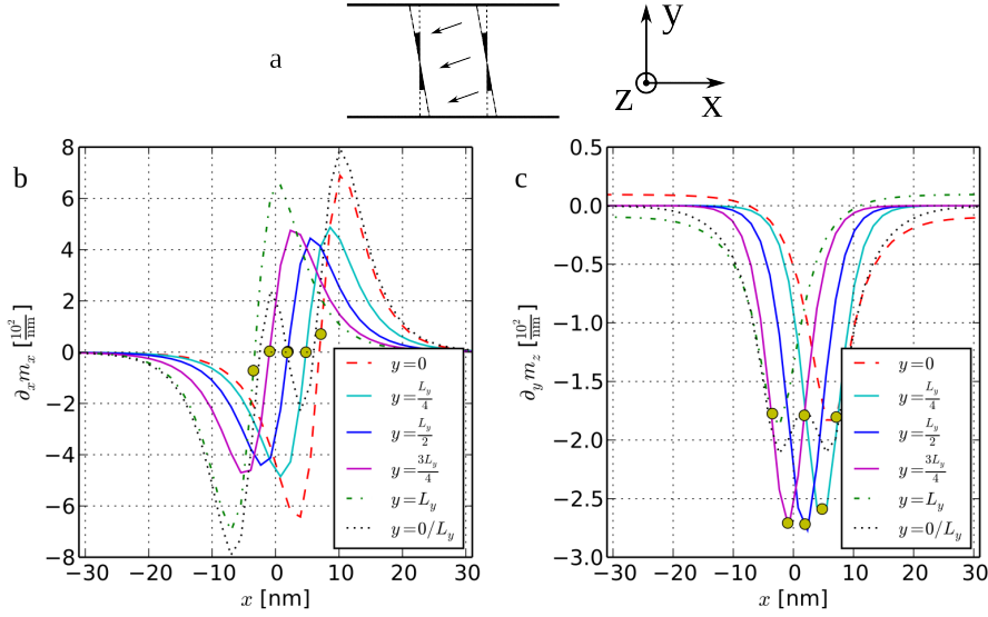
Figure B1. A symmetric DW in an out-of-plane magnetized nanostrip is defined as a DW in which the magnetization, for every y -value (except at the edges) as a function of x with m_z = 0 corresponding to x = 0 , is (i) an odd function when considering the magnetization in the z -direction and (ii) an even function when considering the magnetization in the x - and y -direction. Moreover, the sum of the values at both edges as a function of x should also result in (i) odd or (ii) even functions, respectively. A sketch of a typical symmetric DW is depicted in (a). In (b) and (c), \partial_x m_x(x, y) and \partial_y m_z(x, y) are plotted for y = 0 (bottom nanostrip), y = \frac{L_y}{4} , y = \frac{L_y}{2} (middle nanostrip), y = \frac{3L_y}{4} and y = L_y (top nanostrip) as a function of x in the case that a DW is moved through a nanostrip with D_{\text{DMI}} = 0.4 \text{ mJ/m}^2 , \mu_0 H_{\text{ext},x} = 20 \text{ mT} , \mu_0 H_{\text{ext},z} = 15 \text{ mT} , L_y = 100 \text{ nm} and L_z = 0.6 \text{ nm} . The points that correspond to m_z = 0 are indicated as yellow dots. With respect to these points, curves are (b) odd and (c) even, except at the edges. However, if we sum the values at the edges ( y = 0/L_y ), the resulting curves are also (b) odd and (c) even, indicating that such a DW is symmetric in accordance with what we expect from Fig. 1 (c,d).
