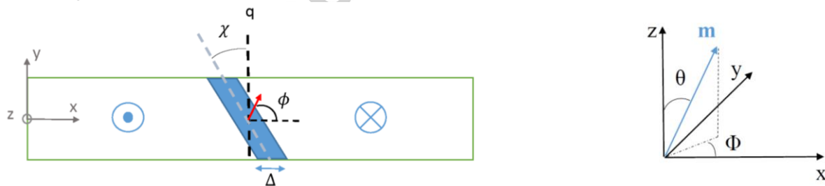
(a) Top view of the nanowire, showing the coordinates q , \Delta and \chi .
