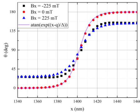
B_x = 0
