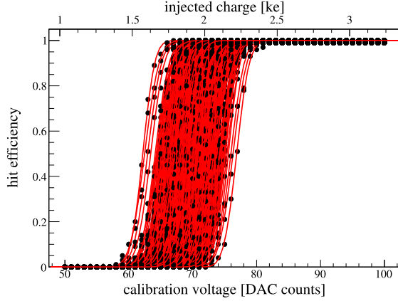
Fig. 9. Calibration voltage scan for all the synchronous front-end pixels.
