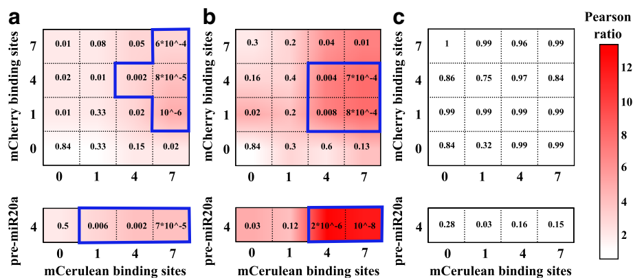
Fig. 5 Fold Pearson and p values. The Pearson ratio is measured for three different values of eYFP basal expression: below threshold (a), around threshold (b), and above threshold (c). p values are reported for each combination of miRNA MREs on the two plasmids. The regions inside the blue perimeters are statistically significant with p < 0.01 . As predicted by the model, the correlation is maximal around the threshold and could be even 12-fold higher than in the unregulated case. Blue-delimited areas are regions whose Pearson ratio (i.e., the ratio of the Pearson coefficients between mCherry and mCerulean possessing different MREs for the same measure in the absence of MREs) is statistically relevant with respect to the corresponding unregulated case. eYFP enhanced yellow fluorescent protein, miRNA microRNA, MRE miRNA regulatory element
