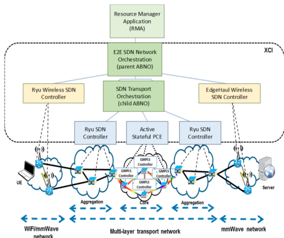
Figure 5: Hierarchical multi-domain resource management.
