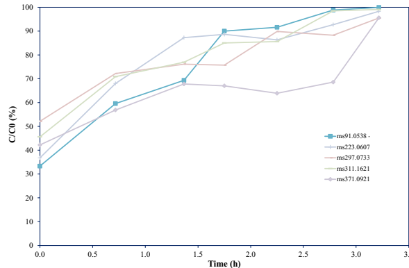
Figure 3 – Siloxane compounds detected during the removal of VOCs – 91.05 C 3 H 10 O 2 SiH+, 223.06 D 3 H+, 297.07D 4 H+, 311.16 L 4 H+, 371.09 D 5 H+.
