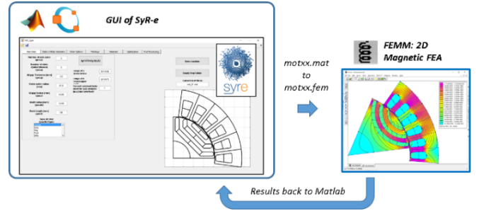
Fig. 1. Principle of operation of SyR-e
