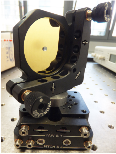
Fig. 2. Back side view of a 2in double sided gold mirror with a 45° central hole; the mirror is mounted on a x-y-z translator for alignment purposes.
