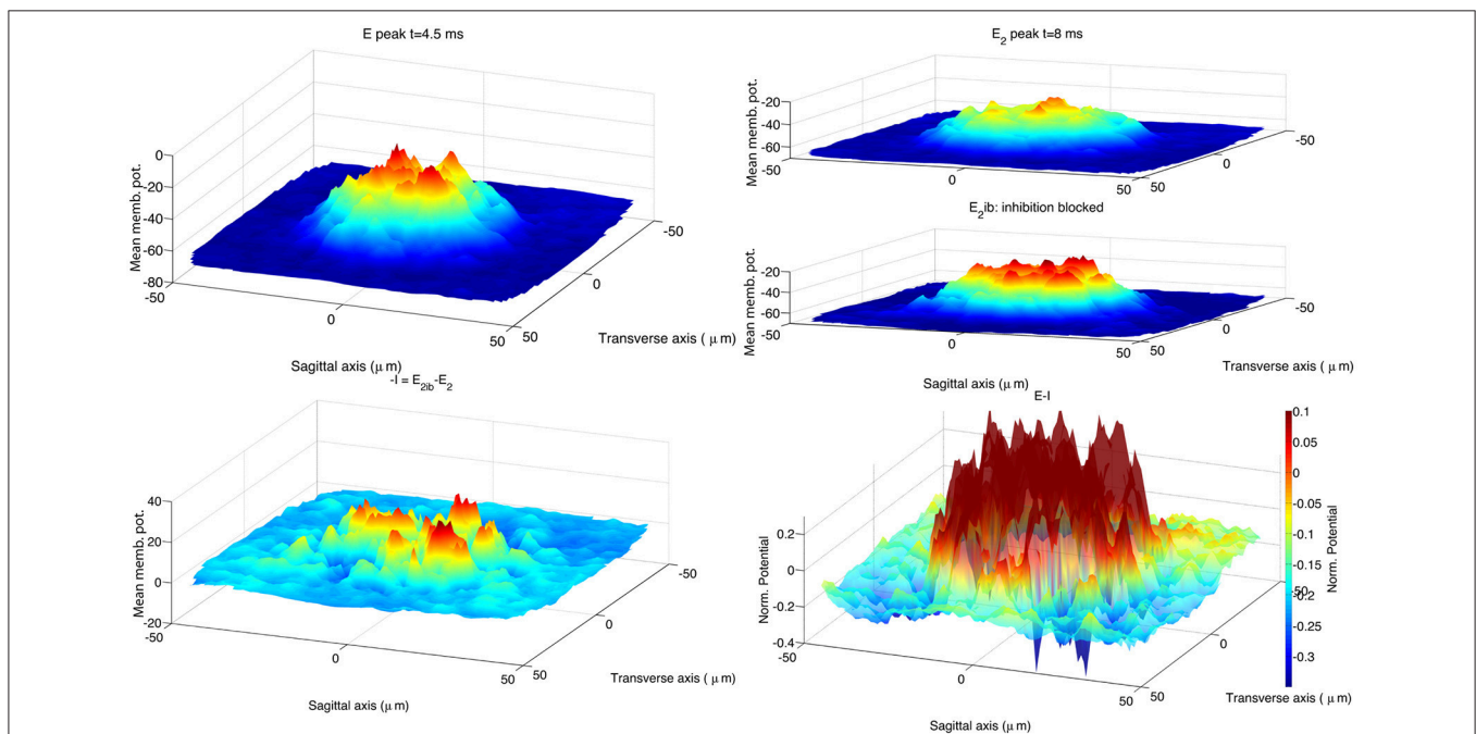
FIGURE 6 | Response of the biologically realistic model (Solinas et al., 2010b) to the activation of 13 MF terminals located within 20\mu\text{m} from the network center. As in the 2010 publication, at the end of each simulation the voltage trace of GrCs aligned along the vertical axis are pooled together to represent their ensemble activity. The resulting 2D surface represents the activity of this 3D GLN network (vertical axes show the mean membrane potential in mV). The simulations in control and partial inhibition block configuration are repeated 10 times, using each time a different network structure. The 2D surfaces belonging to each configuration class are used to build an average response for that class of GLN to the stimulus. The arrangement of data plots replicates the organization of Figure 5 . The activated spot (upper left panel) has a diameter of 36\mu\text{m} if measured at 70% of its peak amplitude (Mapelli et al., 2010b). The stimulus consists in a sequence of 3 spikes with an inter-spike interval of 333 ms. The first peak of GLN activation is reached within 4.5 ms from stimulus onset ( E peak; upper left panel). The GLN shows a second peak of activity E_2 with latency 8.2 ms from stimulus onset (upper right panel). Blocking inhibitory synapses induces a generalized increase of the GLN activity from this time on, note the E_2 peak amplitude and its spatial extension ( E_{2ib} ; upper right panel). The spatial effect of inhibition is calculated as the point difference of the E_2 and E_{2ib} surfaces ( -I ; lower left panel). The center-surround is represented as the difference the surfaces E and the I (lower right panel). The CPU time required to run one of the 20 simulations was 20 min on a Apple® MacBook Pro (Intel Core 2 Duo 2.93 GHz) plus 30 min to process the recorded data.
