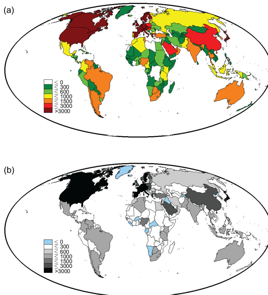
Fig 1. World map of the water suitcase. (a) The water suitcase of emigrants from each country in 2010 and (b) water suitcase variations from 1990 to 2010; suitcases and variations are measured in \text{m}^3 per capita per year.
