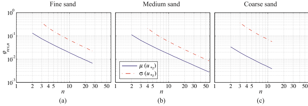
Figure 5: Convergence of the the mean \mu(u_{st}) and standard deviation \sigma(u_{st}) for each sub-ensemble (fine, medium and coarse sand)
