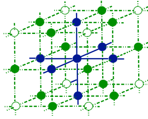
Figure 3. Oscillations in the infinite weak component.
