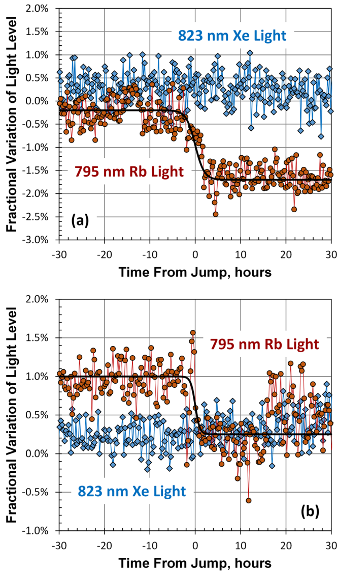
FIG. 8. Two examples of lamplight intensity jumps observed in the laboratory from a study aimed at measuring the Rb consumption rate for GE-180 glass. The solid line through the 795 nm Rb light intensity is a logistic function (i.e., S_{795}(t) = S_0 + \delta S / (1 + e^{t/\tau}) ), whose parameters \delta S and \tau characterize the jump: for the jump in (a) we have \delta S = 1.5\% and \tau = 1 h, while for the jump in (b) we have \delta S = 0.75\% and \tau = 0.5 h.
