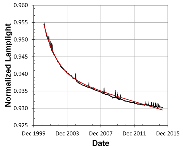
FIG. 3. Multiyear trend of normalized lamplight intensity (i.e., light level telemetry) from the RAFS onboard GPS SVN-54. The smooth line through the data is a fit to the form of Eq. (10).
