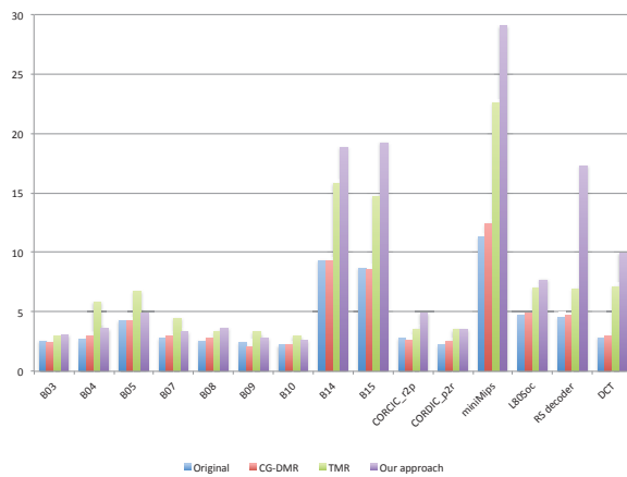
Fig. 7. Clock period comparison for the considered circuits using different error detection and correction approaches.
