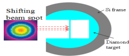
Figure 2. Scheme of the C-shaped support of the target.
