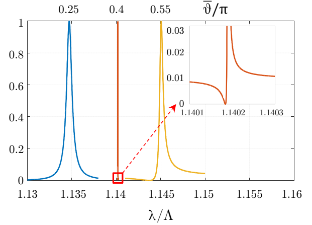
Fig. 11. Cuts of the reflectivity map reported in Fig. 8 for t_g = 0.9\Lambda (blue), t_g = 0.95\Lambda (red), t_g = \Lambda (orange). A zoom on the red curve is used to highlight its very quick zero-one transition. At top, the normalized \bar{\vartheta} values of the peaks are reported to establish the correspondence with Fig. 10.
