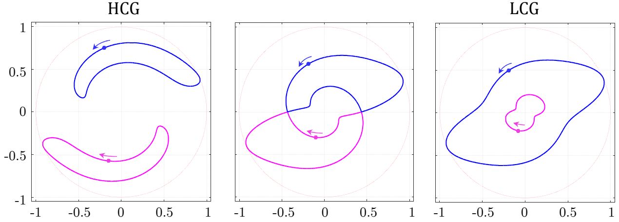
Fig. 6. Parametric study of the half loop gain eigenvalues \lambda_i(\Delta\vartheta) for \Phi = 33.26^\circ , \Psi = 246.02^\circ (as in Fig. 4) and \Delta\vartheta \in [0, 4\pi] . The left, center and right figures refer to \Theta = 62.55^\circ (corresponding to a HCG), \Theta = \Theta_c = 79.15^\circ (obtained from (15)), \Theta = 83.00^\circ (corresponding to a LCG). The blue and magenta curves are the orbits of the two eigenvalues in the complex plane. The points mark the \Delta\vartheta = 10.00^\circ position and the arrows indicate the direction of motion for increasing \Delta\vartheta . Note that in all cases the trajectories are tangent to the unit circle, drawn in red.
