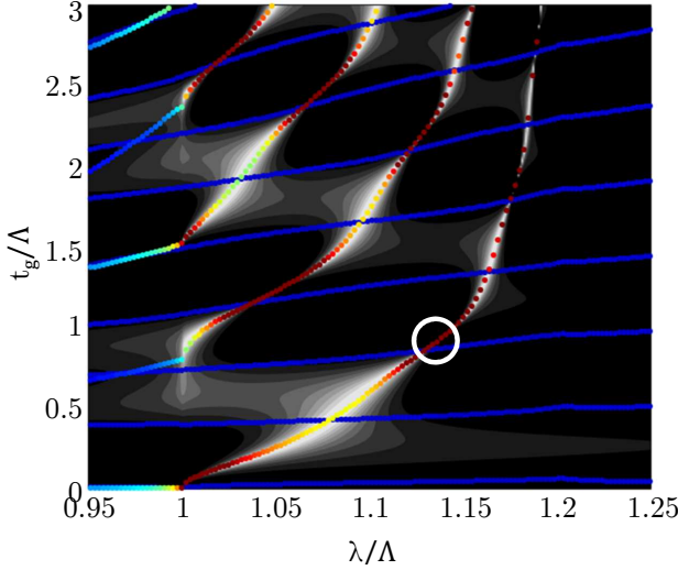
Fig. 8. TE reflectivity map for normal-incident plane-wave (linear, gray scale: brighter regions indicate high reflectivity) of a low-contrast grating in the (\lambda, t_g) plane. The grating consists of \text{SiO}_2 bars ( n_1 = 1.45 ) surrounded by air, \eta = 60\% . The resonance curves are superimposed and their color quantifies the resonance quality factor (blue low, red high). The marker indicates the point U ( \lambda = 1.141\Lambda , t_g = 0.95\Lambda ), where Q \rightarrow \infty .
