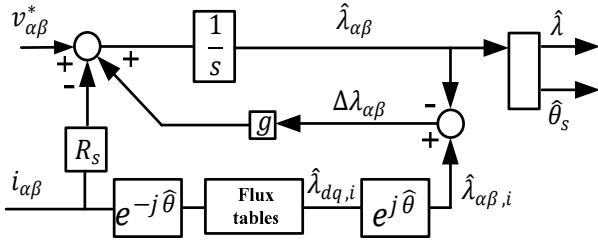
Fig. 3. Stator flux observer.
