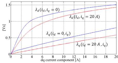
Fig. 4. Flux linkage maps of the SyRM under test, evaluated experimentally.
