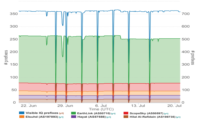
Figure 10: Visible Iraqi prefixes (June, 20- July, 2015). Number of prefixes observable in BGP that geolocate to Iraq (blue line, y_2 axis) and number of unique prefixes announced by the 5 top Iraqi providers (stacked lines, y_1 axis). An observable series of \approx 3 -hour outages starts on June 27, and ends on July 15. According to the media, the local government ordered complete shutdowns of the Internet service in the country.
