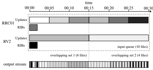
Figure 3: Intra- and inter-collector sorting in libBGPStream. An example showing how RIB and Updates dumps generated by a RIPE RIS collector (RRC01) and a RouteViews collector (RV2) are interleaved into a sorted stream. The 30 minutes (10 files) of BGP data are first separated into two disjoint sets (of 6 and 4 files) based on overlapping file time intervals. Then a multi-way merge is applied separately to the two sets, yielding the stream depicted at the bottom.
