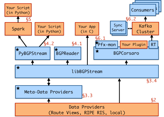
Figure 2: BGPStream framework overview. Blue boxes represent components of the framework; those marked with a star are distributed as open source in the current BGPStream release [11]. Orange boxes represent external projects or placeholders. Section numbers mark where each component is discussed in this paper.
