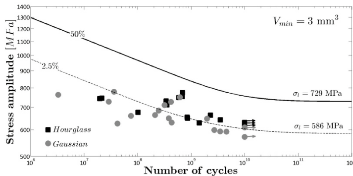
Fig. 5. P-S-N curves estimated at the smallest V_{real} .
