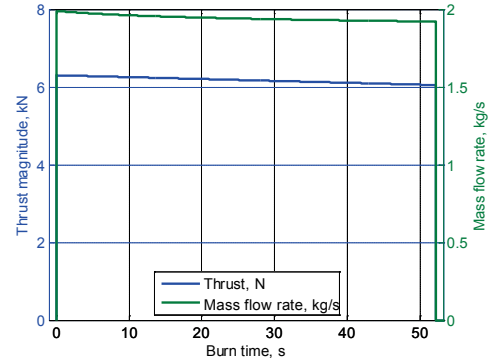
Fig. 5: Thrust profile for the DEO-Kit disposal.
