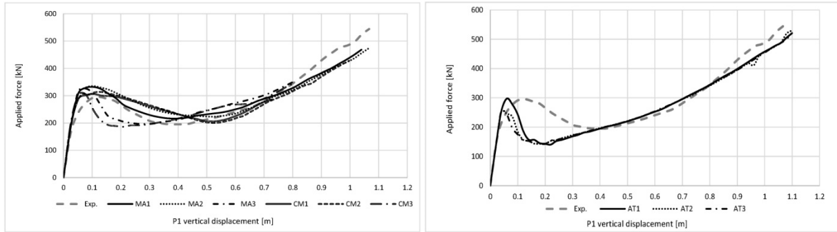
Fig. 2. (a) P1 vertical displ. – Applied force (SeismoStruct); (b) P1 vertical displ. – Applied force (ATENA 2D);
