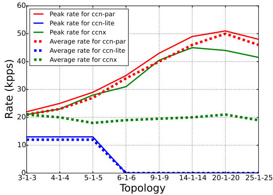
Fig. 4: Packet forwarding rate.
