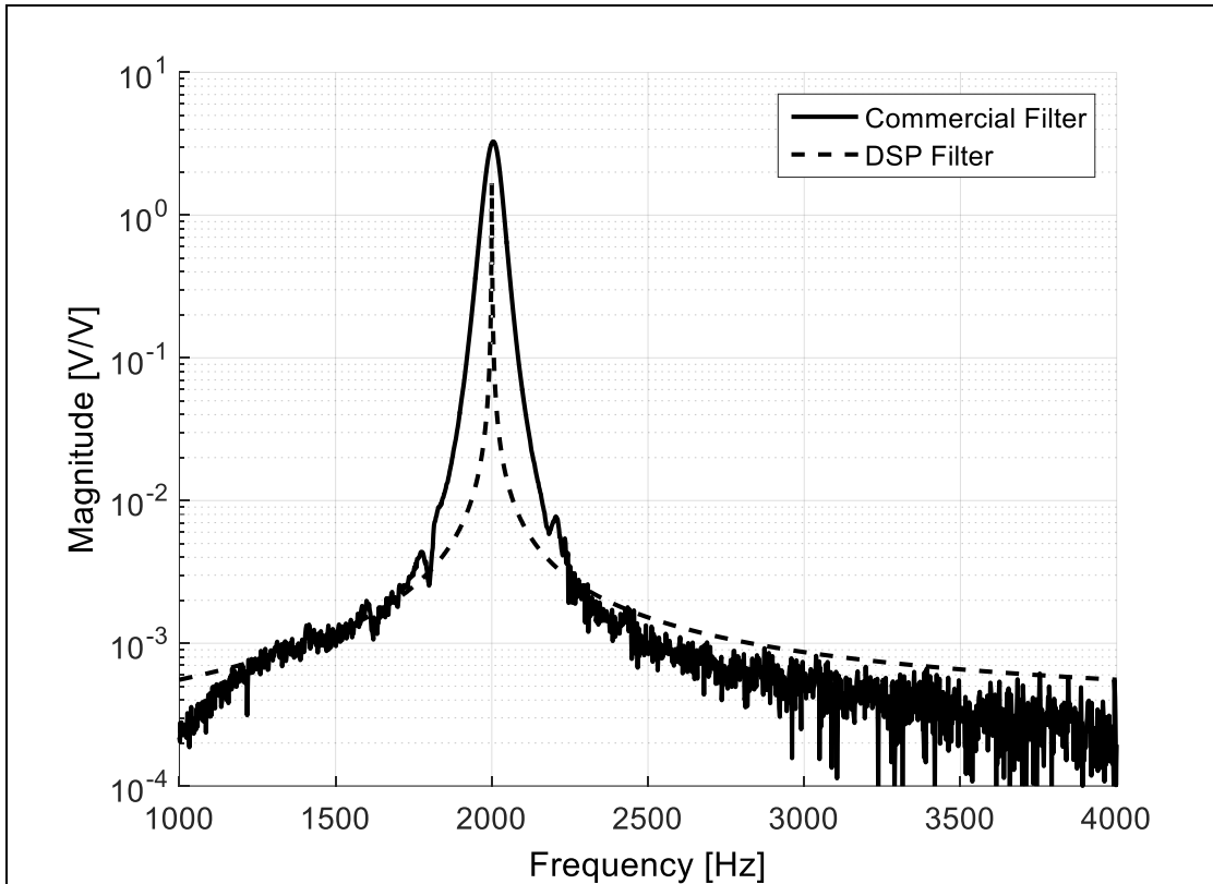
Figure 6: Comparison between the Commercial filter Transfer function and the DSP implemented
