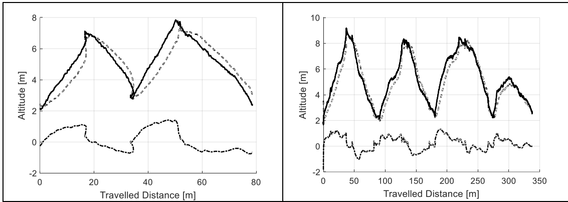
Figure 8: Terrain following performances - solid line: terrain profile, dashed line: flying altitude reported to ground (current altitude – imposed distance (5m)), dash-dot line: absolute error
