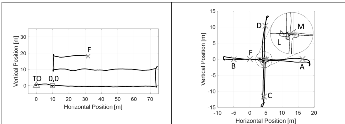
Figure 9: Acquired GRID (left) and CROSS (right) flight path
