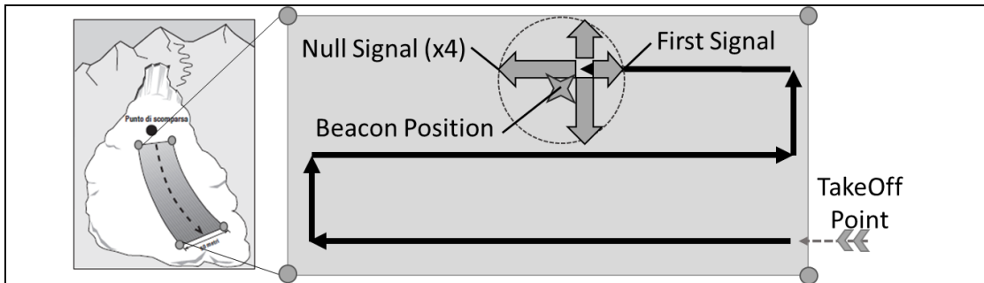
Figure 7: Search scheme: Solid Arrow – GRID Flight, Thick Arrow – CROSS Flight
