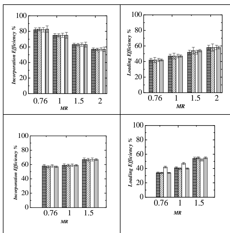
Fig. 2. Menthol Loading and Incorporation efficiency (%) of menthol with (▨ ▩) CIJM mixer MIVM-2(□ ▣) mixers. Operating conditions, quench volumetric ratio=1. [Above at ( C_p = 6 \text{ mg ml}^{-1} (M.R 0.76, c_{\text{menthol}} = 4.56 \text{ mg ml}^{-1} ), (M.R 1, c_{\text{menthol}} = 6 \text{ mg ml}^{-1} ), (M.R 1.5, c_{\text{menthol}} = 9 \text{ mg ml}^{-1} ), (M.R 2, c_{\text{menthol}} = 12 \text{ mg ml}^{-1} )] [Below at ( C_p = 12 \text{ mg ml}^{-1} (M.R 0.76, c_{\text{menthol}} = 9 \text{ mg ml}^{-1} ), (M.R 1, c_{\text{menthol}} = 12 \text{ mg ml}^{-1} ), (M.R 1.5, c_{\text{menthol}} = 18 \text{ mg ml}^{-1} ), Flow rates =20, 80 ml min -1
