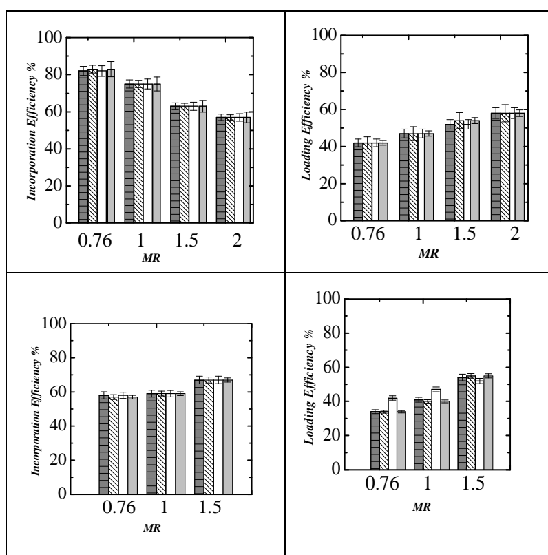
Fig. 2. Menthol Loading and Incorporation efficiency (%) of menthol with (▨▩) CIJM mixer MIVM-2(□▣) mixers. Operating conditions, quench volumetric ratio=1. [Above at ( C_p = 6 \text{ mg ml}^{-1} (M.R 0.76, c_{\text{menthol}} = 4.56 \text{ mg ml}^{-1} ), (M.R 1, c_{\text{menthol}} = 6 \text{ mg ml}^{-1} ), (M.R 1.5, c_{\text{menthol}} = 9 \text{ mg ml}^{-1} ), (M.R 2, c_{\text{menthol}} = 12 \text{ mg ml}^{-1} )] [Below at ( C_p = 12 \text{ mg ml}^{-1} (M.R 0.76, c_{\text{menthol}} = 9 \text{ mg ml}^{-1} ), (M.R 1, c_{\text{menthol}} = 12 \text{ mg ml}^{-1} ), (M.R 1.5, c_{\text{menthol}} = 18 \text{ mg ml}^{-1} ), Flow rates =20, 80 ml min -1
