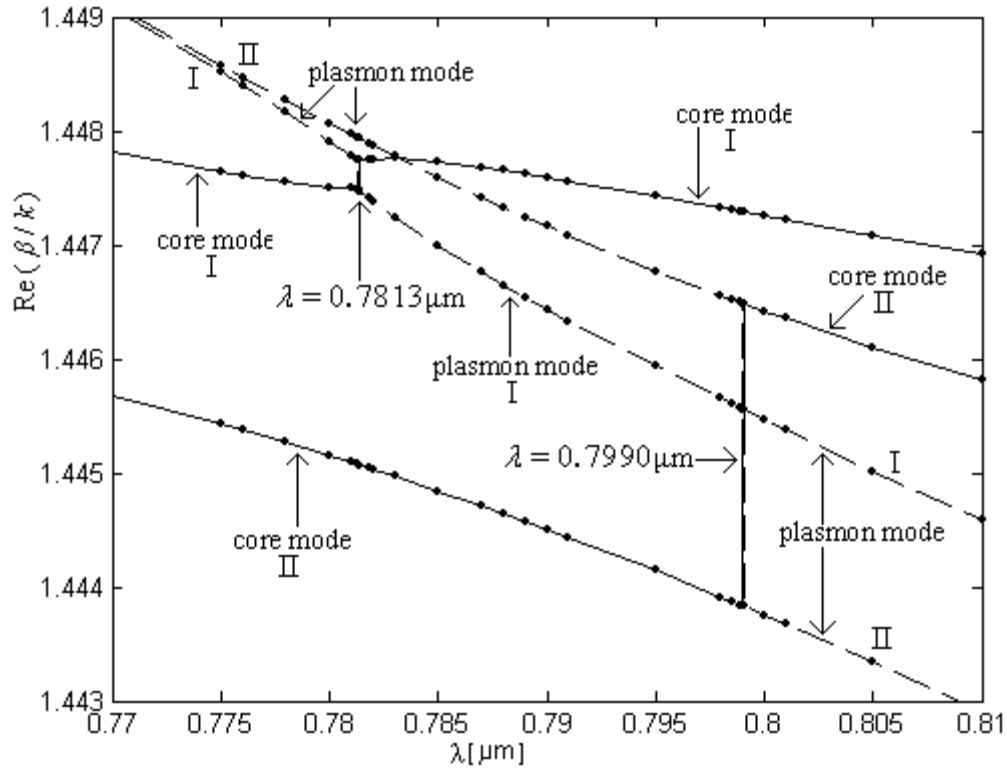
Fig. 4. The real part of the effective index versus the wavelength for the core and plasmon modes near the loss matching point ( \lambda_I = 0.78135 \mu m and \lambda_{II} = 0.7990 \mu m ) for a photonic crystal fiber ( r_1 = r_2 = \dots = r_{14} = 0.5 \mu m , r_{15} = 5 \mu m , r_{16} = 5.04 \mu m and d = 2 \mu m ) when the refractive index of the analyte is n_a = 1.39 .
