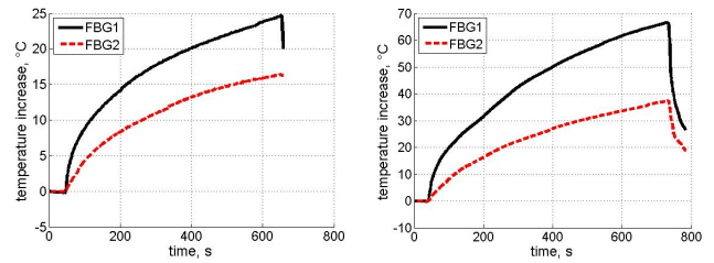
Fig. 5 Temperature evolution recorded by FBGs inside porcine liver during 2W (left) and 4W (right) of laser ablation. FBG1 is aligned with the area of maximum laser irradiation and FBG2 is 2cm away.
