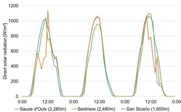
Figure 13 – Direct solar radiation for some sites compared with the test site (9-11 June 2016).
